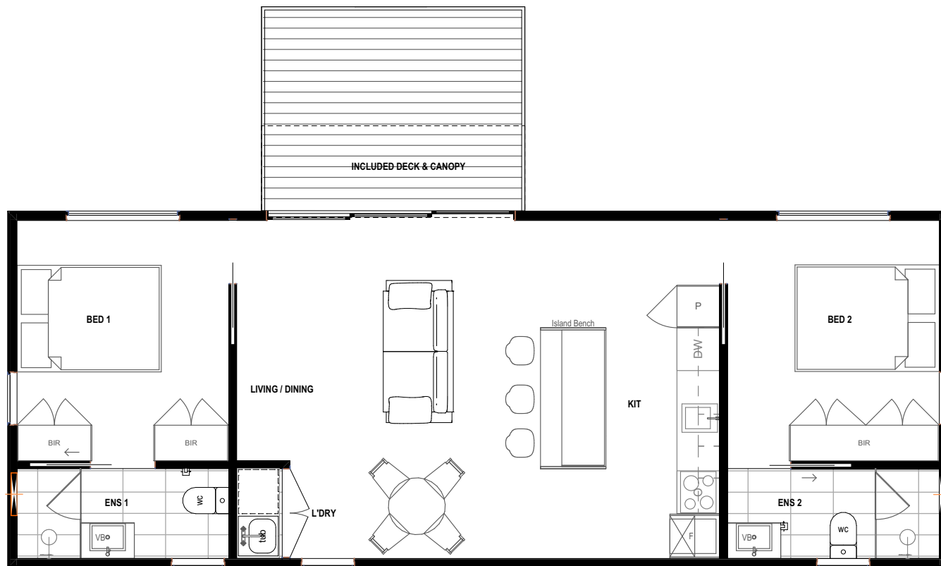
FLOOR PLAN
