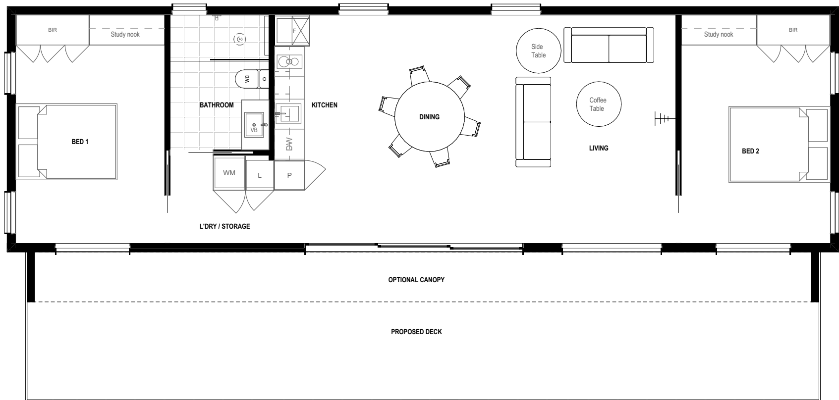
FLOOR PLAN
